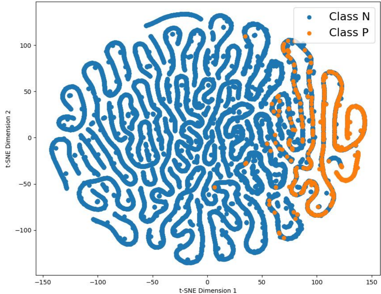
t-SNE Visualization of Embeddings
